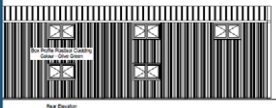
Rear Elevation
